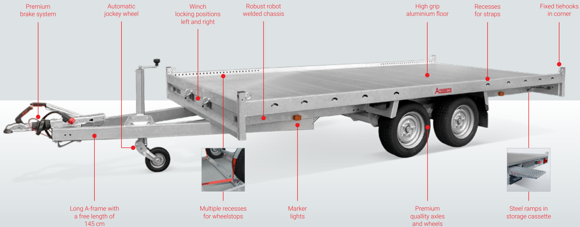
Aluminium floor and fixed tiehook in corner
